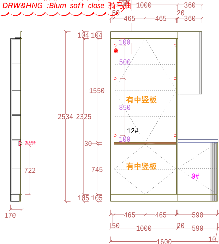
SECTION VIEW 1
