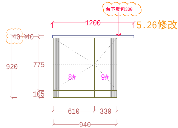
ELEVATION F
