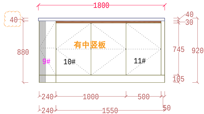
ELEVATION D
