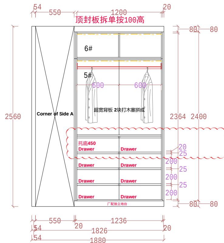
INNER VIEW B
