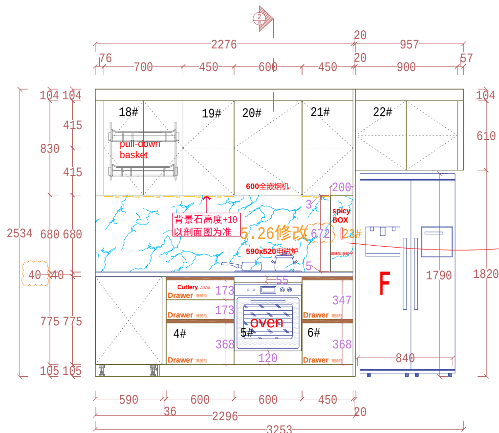
ELEVATION C
