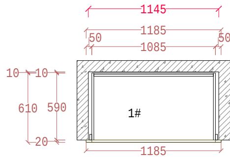
PLAN VIEW floor
