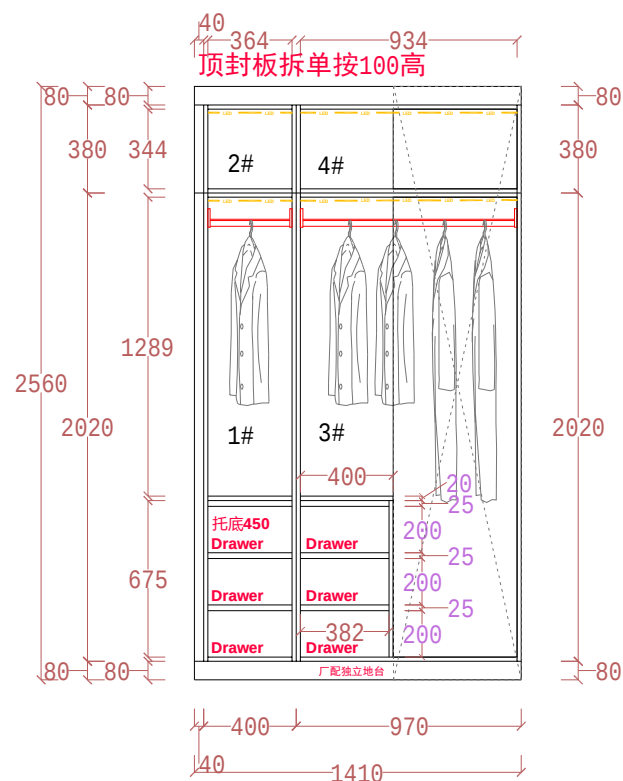
INNER VIEW A
